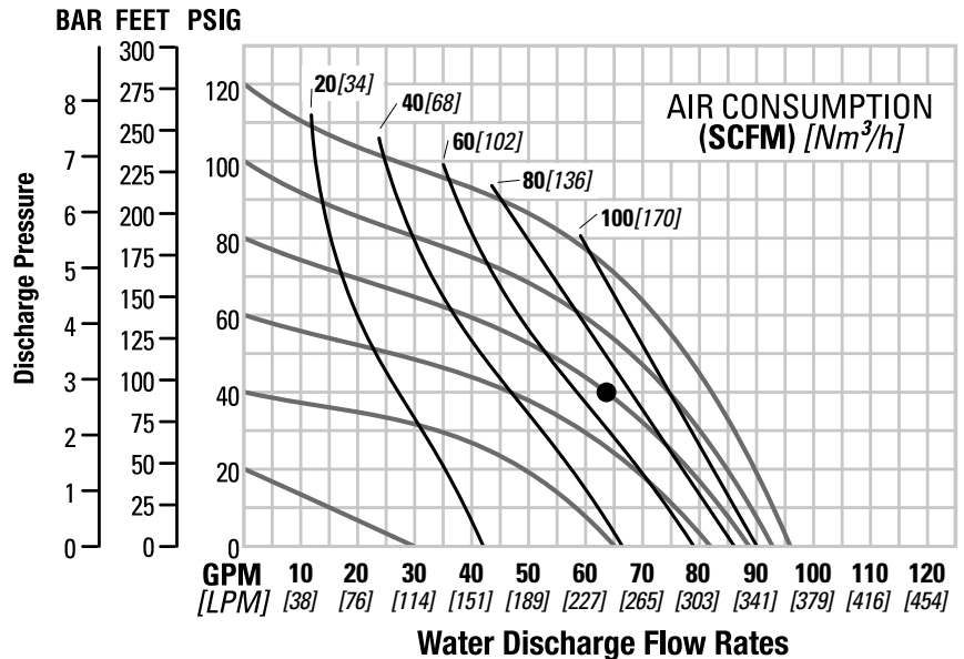
Flow rates indicated on chart were determined by pumping water. For optimum life and performance, pumps should be specified so that daily operation parameters will fall in the center of the pump performance curve.
