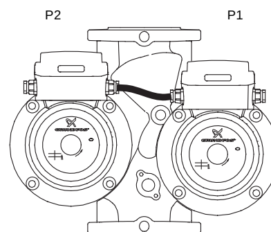
Fig. 6 Twin-head pump
