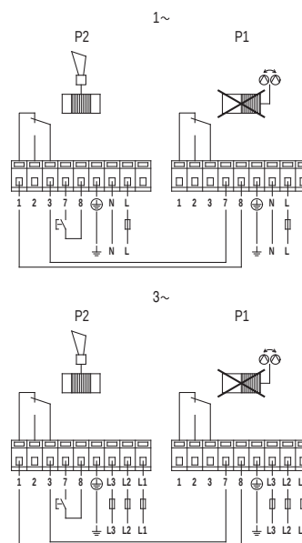
Fig. 19 Standby operation
